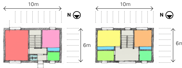
B2. Rectangular 2 bedroom house, with its long side facing the street and street access on the opposite facade to the main solar incidence facade
