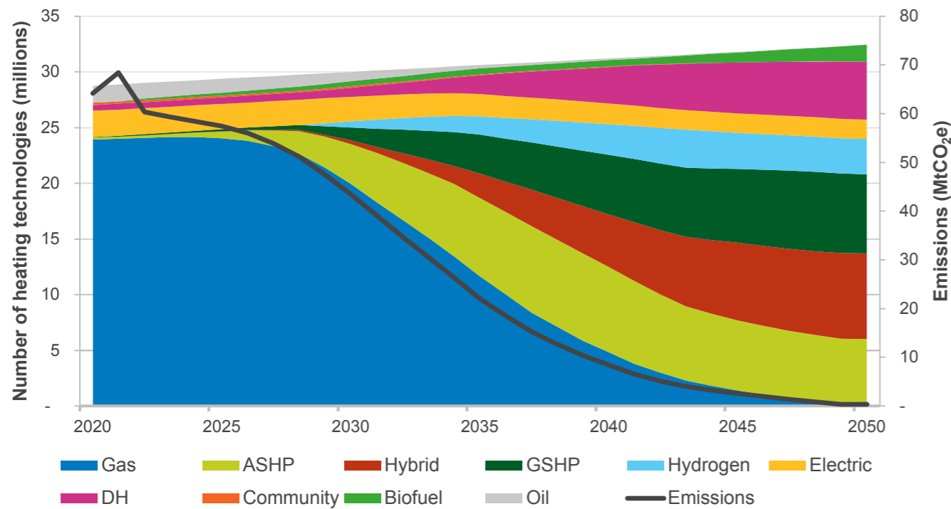
Figure NZ.24: Estimated number of heating technologies and the associated emissions reduction to 2050 in Leading the Way
